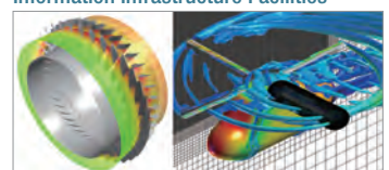
CFD analysis examples (aeroengine compressor turbine blades/ interference between helicopter fuselage and rotors)
