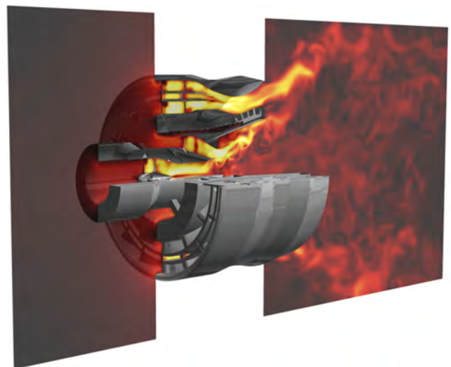
Mach number distribution of the aeroengine fuel nozzle analysis performed with engine combustion simulation software "HINOCA"
