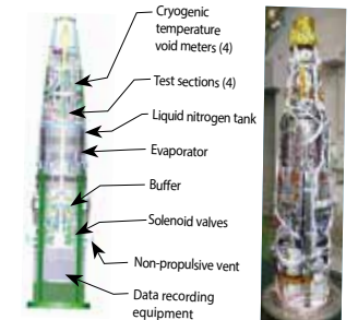
Cryogenic temperature test equipment loaded onto the sounding rocket
