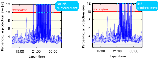
The results of a simulation using the hybrid technology; the amount of time without access to satellite navigation that exceeds the warning level (the red line) is 1.92% with the conventional approach (left) but just 0.8% (half the amount under the conventional approach) with the hybrid technology (right).
