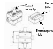
Overview of the cryogenic void meter
