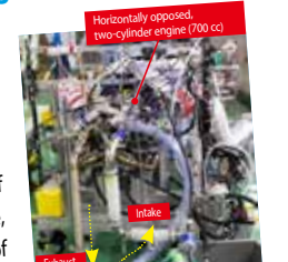
Equipment for testing high-altitude, turbocharged engines using a reciprocating engine
