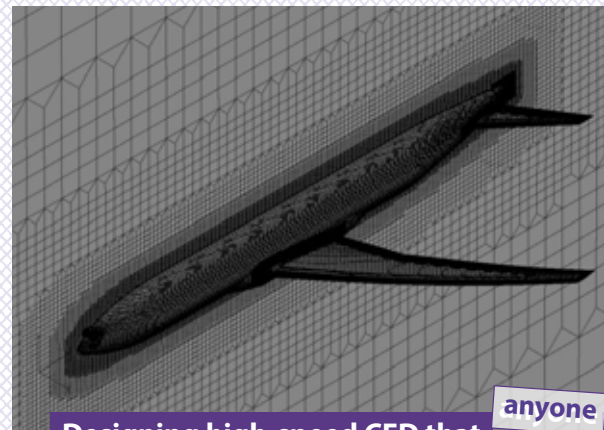
A computational grid created with HexaGrid
