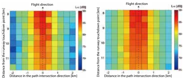
The measured aircraft noise (left) nearly matches the predicted value (right), proving high prediction accuracy. Deeper red colors correspond to higher noise levels.
