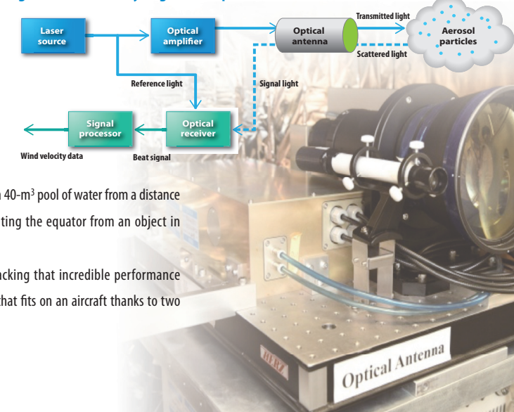
Figure 3: The heterodyning technique
