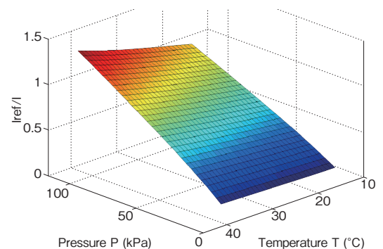
Figure 4 Example of PSP pressure and temperature characteristics
