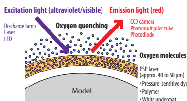
Figure 2 PSP structure
