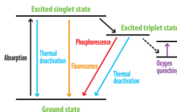
Figure 3 Reaction process for photoexcitation molecules
