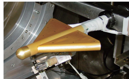
Figure 5 Wind tunnel model with AA-PSP coating
