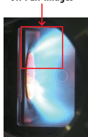
Combustion instability experiment at the high-temperature and high-pressure combustion test facility (Inlet pressure: 7 bar, Inlet temperature: 760 K). Time-series OH-PLIF images during a transition to combustion instability. The images were measured by the high-speed OH-PLIF at an interval of 1/10,000 of a second.
