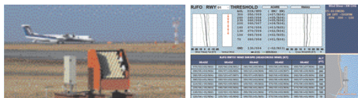
L: A SOLWIN Sodar (the red box in the middle-foreground area) in a trial setup at Oita Airport
