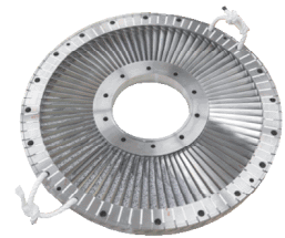
A low-pressure turbine prototype for flutter testing
