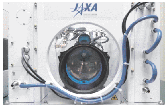
The developed turbulence detection system is light and compact enough for mounting on passenger aircraft
